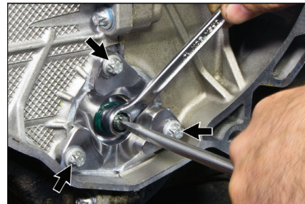
Intermediate shaft (IMS) bearing replacement. 15 Cylinder Head
