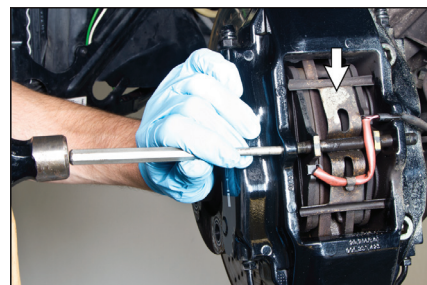
Step-by-step brake pad, pad sensor and rotor replacement. 46 Brakes-Mechanical
